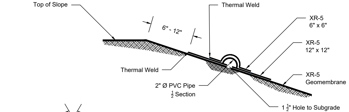
Pipe Vent Cross Section
